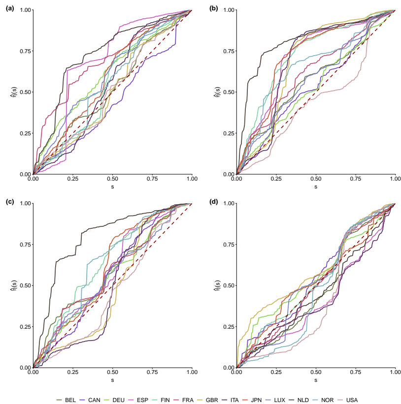
Figure 4. Estimated variance profiles for year-on-year inflation rates of selected OECD countries: (a) February 1957–September 1994, monthly CPI data from Culver and Papell (1997) . Other panels: monthly CPI data from the OECD database for (b) April 1961–March 2019 (c) April 1961–December 1989 (d) January 1990–March 2019.
