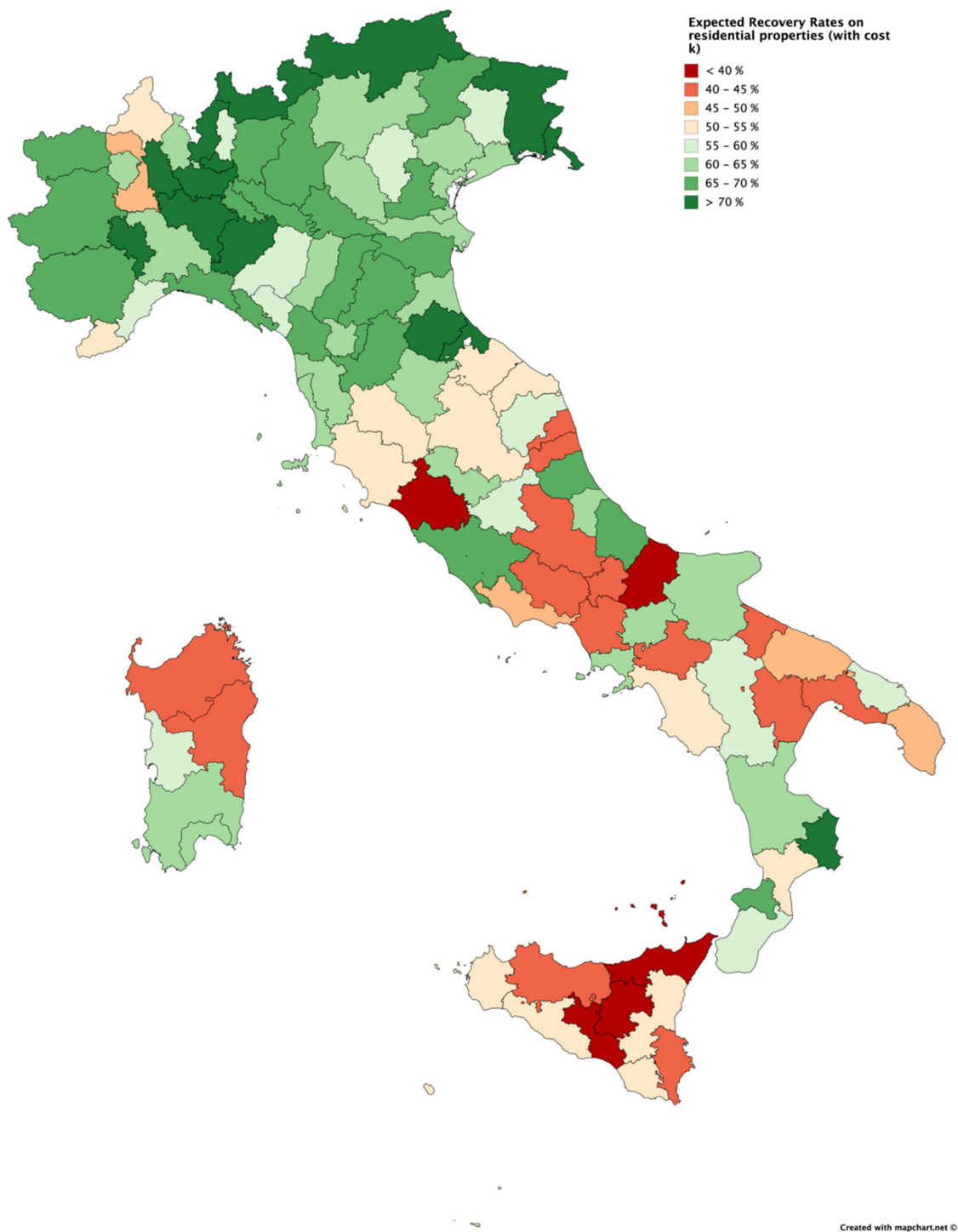
Figure 2. Expected recovery rates for residential properties. (Mapchart.Net 2020).
