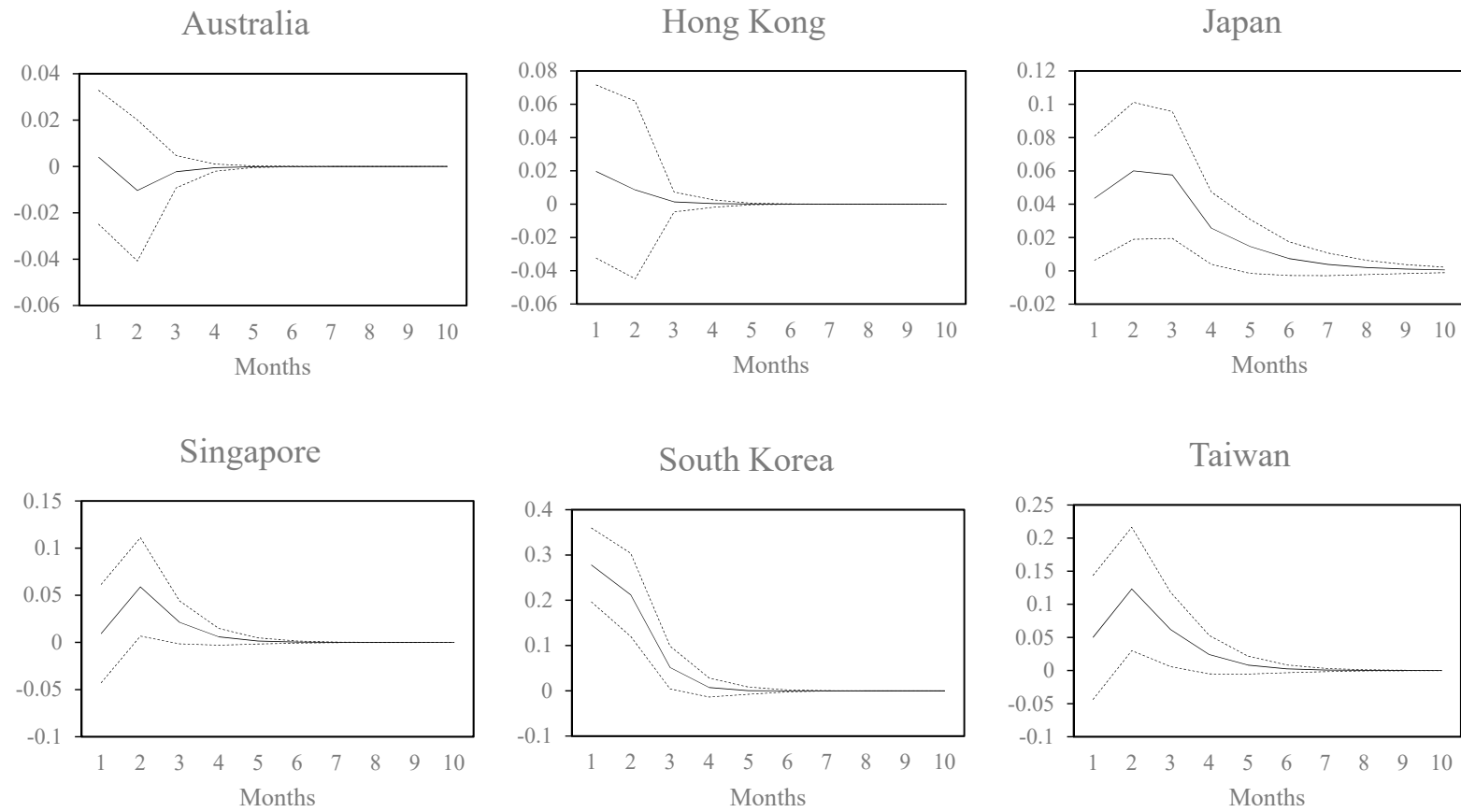
Figure 2. Impulse response functions (IRFs) of TURN to RET with two standard error bands. Note: For each market, the solid line is the impulse response function of TURN to RET following a one- SD RET innovation; the two dashed lines are the confidence bands of two standard errors.
