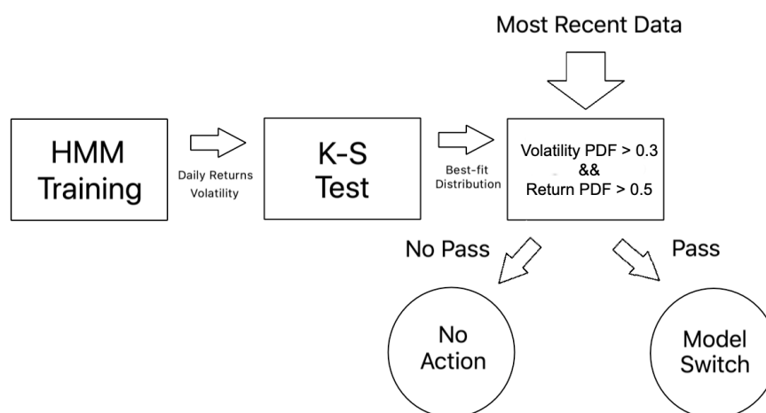
Figure 5. Diagram overview of our trading model.
