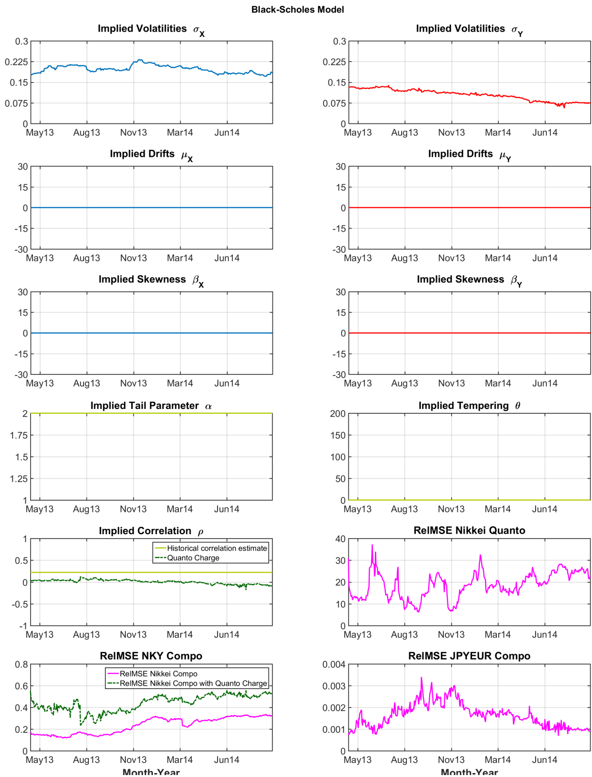
Figure 9. Quanto and compo options: daily calibrated Black–Scholes parameters and RelMSEs. Sample period 16 April 2013 to 15 September 2014.
