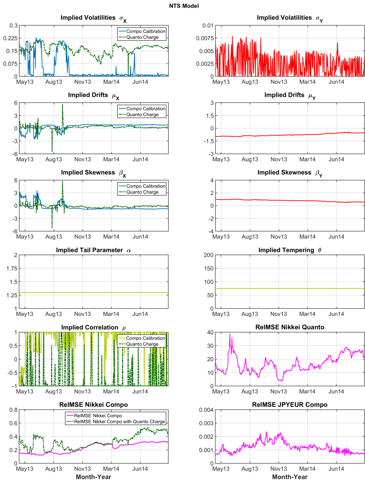
Figure 10. Quanto and compo options: daily calibrated (X, Y) NTS parameters and ReIMSEs. Sample period 16 April 2013 to 15 September 2014.
