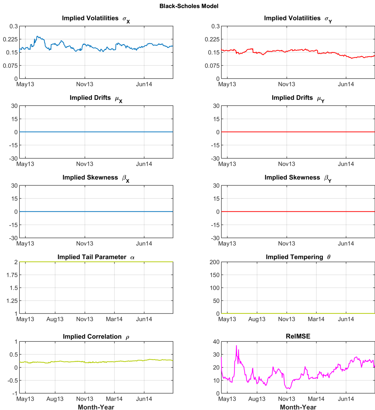
Figure 5. Quanto Calls: daily calibrated Black–Scholes parameters and ReIMSE. Sample period 16 April 2013 to 15 September 2014.
