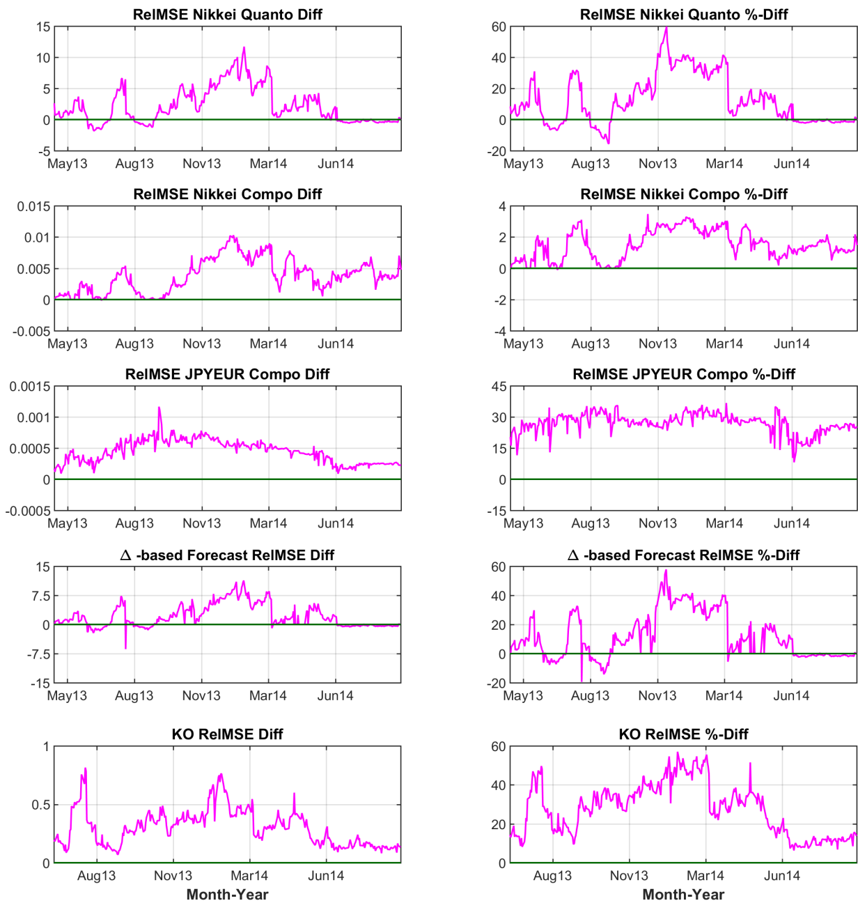
Figure 11. Quanto, compo and KO options. Top three: ReIMSE-difference for the quanto Nikkei, compo Nikkei and JPYEUR options. Bottom two: ReIMSE-difference of the delta-based forecasts of quanto Nikkei call prices and ReIMSE-difference for KO options. Sample period for vanilla options 16 April 2013 to 15 September 2014, for KO options 19 June 2013 to 15 September 2014. Positive values indicate better performance of the NTS model.
