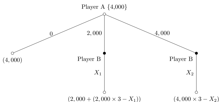
Figure 1: Decision tree
