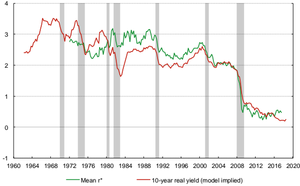
Figure 2: Average r^* and the model implied 10-year real yield
