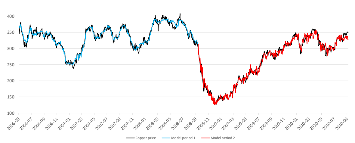
Figure 2. Comparison between the model outputs and the copper prices.
