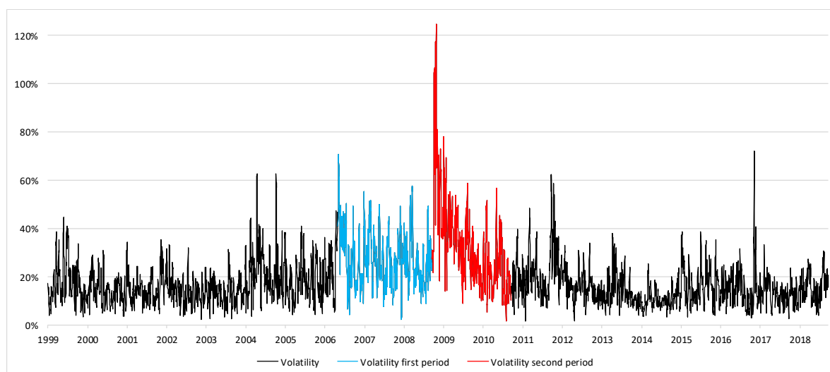
Figure 1. Five-day rolling window copper return annualized volatility from 1999 to 2018.
