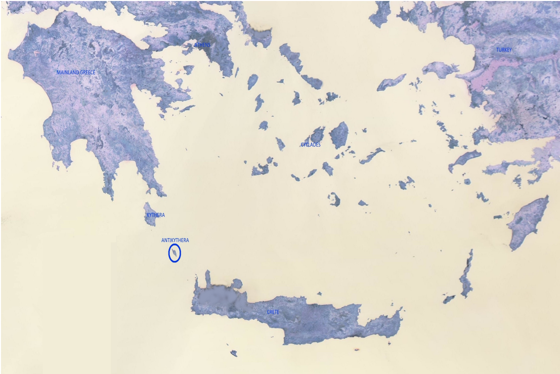
Figure 1: The Mediterranean (original image courtesy of NASA Terra-MODIS)
