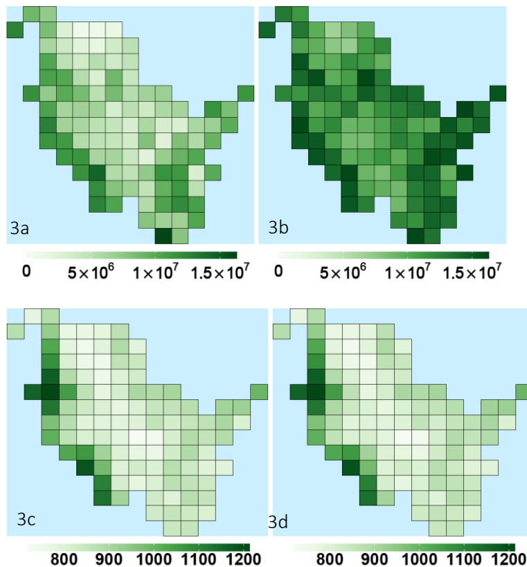
Figure 3: Conservation potential (= modelled number of grasshoppers per km 2 in the climate cell in the absence of any land-use induced mortality) for the first period 2020-2039 (Fig. 3a), and the second period 2060-2079 (Fig. 3b), and the average annual costs in euro of measure M1a of a climate cell for the first period 2020-2039 (Fig. 3c) and the second period 2060-2079 (Fig. 3d). Each grid cell represents a 12x12km climate cell.
