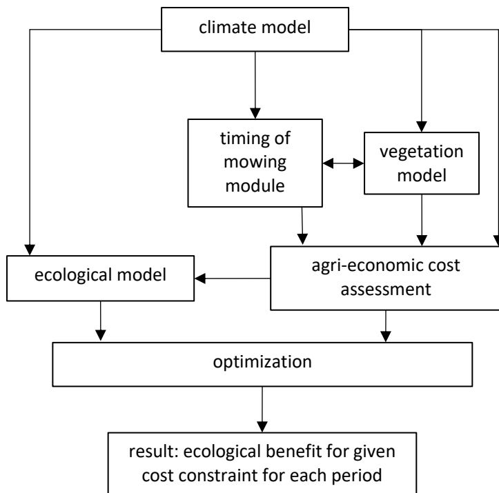
Figure 1: Overview of the climate-ecological-economic model
