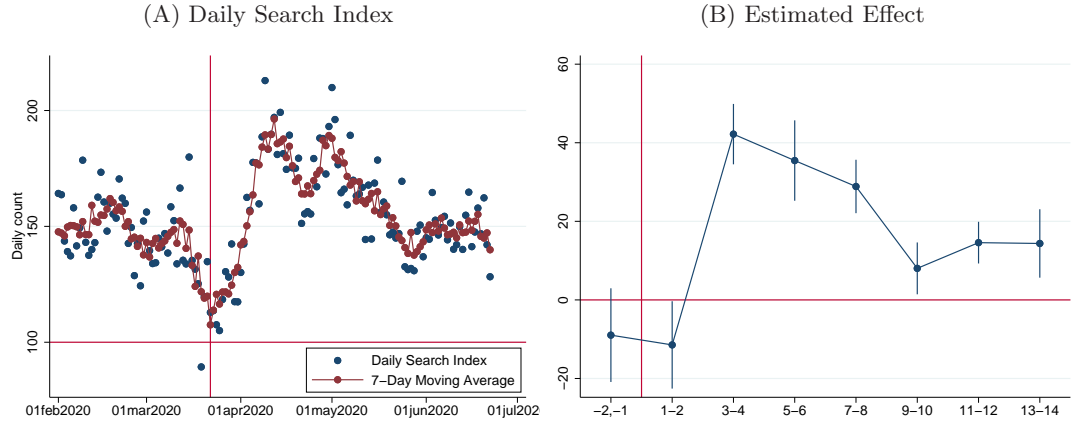
Figure 2: Daily values of the composite index of DV-related search intensity since February 2020 and estimated bi-weekly effects of lockdown
