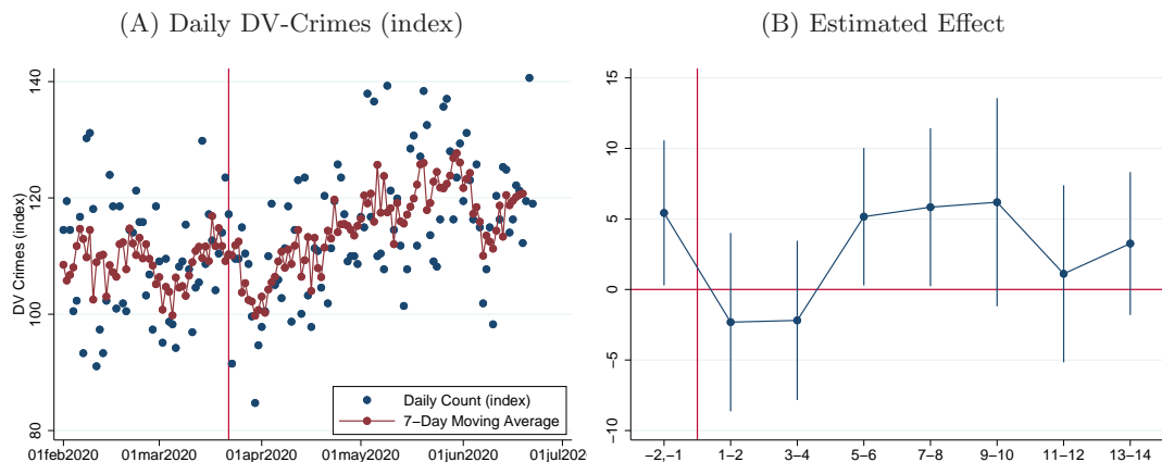
Figure 1: Daily DV-crimes since February 2020 and estimated bi-weekly effects of lockdown
