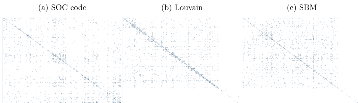
Figure 3: Involuntary occupational-mobility network adjacency matrix
