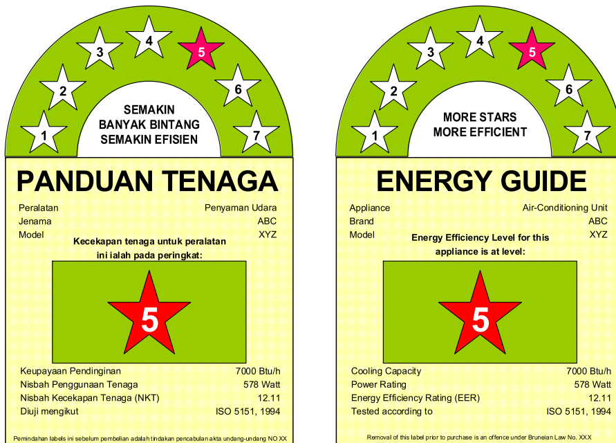
Fig. 3. Label type B in the Malay and English languages.
