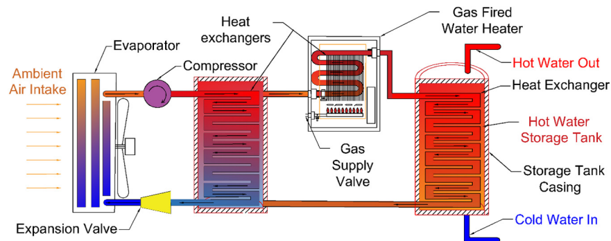
Fig. 14. Schematic diagram of the hybrid gas-fired heat pump water heater (GHFPH).
