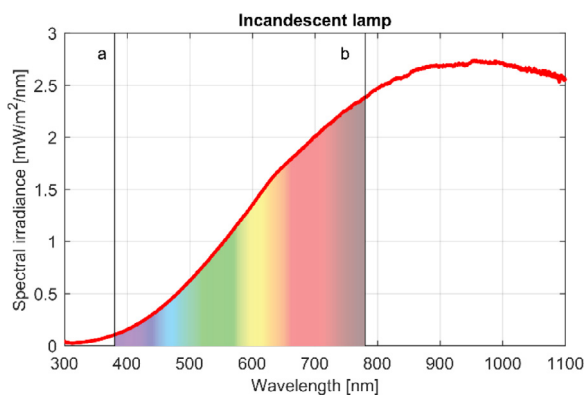
Fig. 11. Halogen incandescent lamp spectrum.
