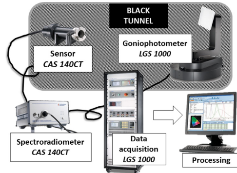
Fig. 6. Measurement scheme in the spectroradiometer.
