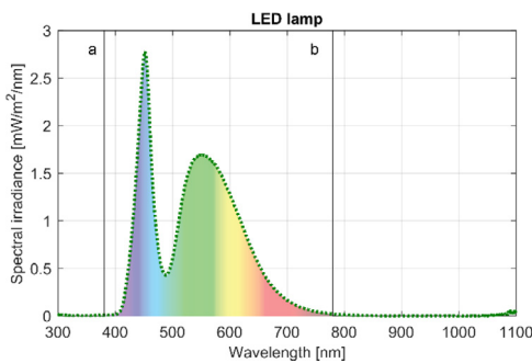
Fig. 15. LED lamp spectrum.
