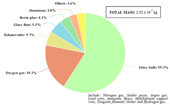
Fig. 27. Halogen incandescent lamp assembly: material input. Based on U.S. Department of Energy (2012) mixture of materials.
