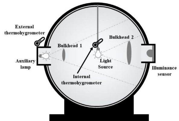
Fig. 10. Schematic of an integrating sphere of Ulbricht.
