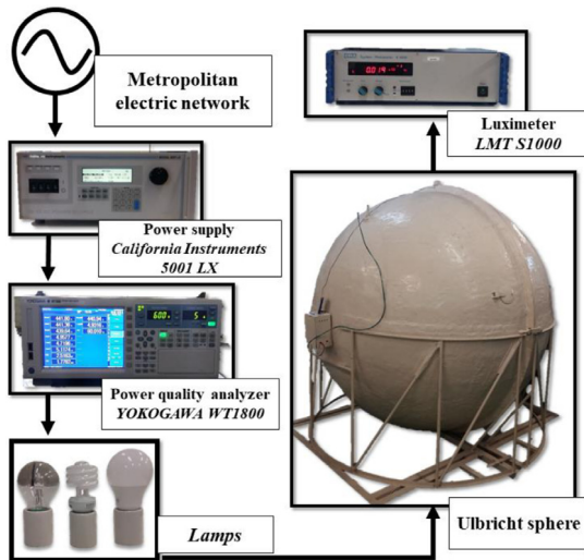
Fig. 5. Measurement scheme for electrical quantities and luminous flux.
