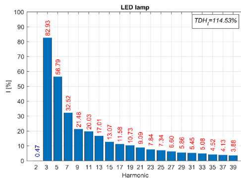
Fig. 23. Harmonic content for the LED lamp.
