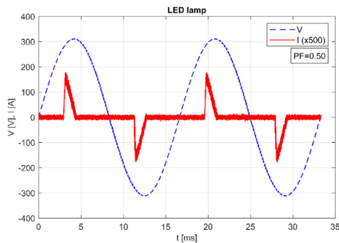
Fig. 22. Voltage and current waveforms for the LED lamp.
