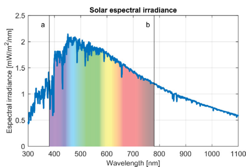
Fig. 2. Sunlight spectral energy emission curve with a color temperature of 6500 K; sun at midday (Tawfik et al., 2018).
