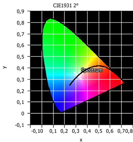
Fig. 16. Chromaticity coordinates for the LED lamp.
