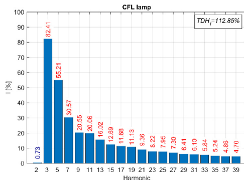
Fig. 21. Harmonic content for the halogen CFL lamp.
