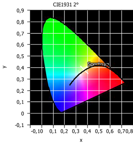
Fig. 14. Chromaticity coordinates for the CFL lamp.
