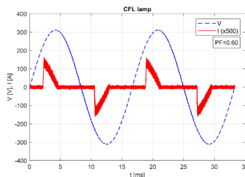
Fig. 20. Voltage and current waveforms for the CFL lamp.
