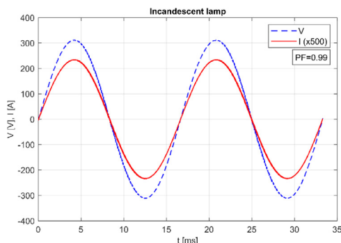
Fig. 18. Voltage and current waveforms for the halogen incandescent lamp.
