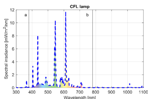
Fig. 13. CFL lamp spectrum.
