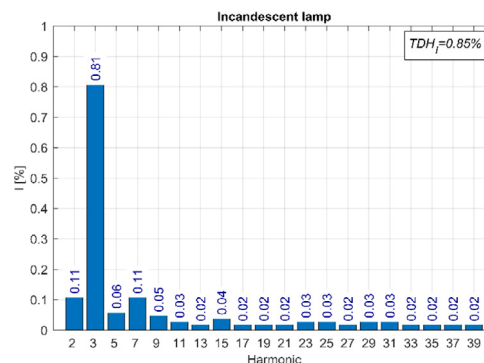
Fig. 19. Harmonic content of the halogen incandescent lamp.
