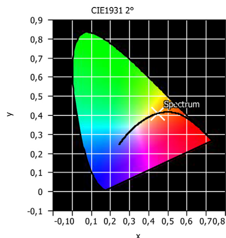
Fig. 12. Chromaticity coordinates for the halogen incandescent lamp.
