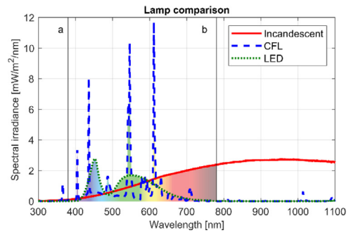
Fig. 17. Comparison between the lamp spectra.
