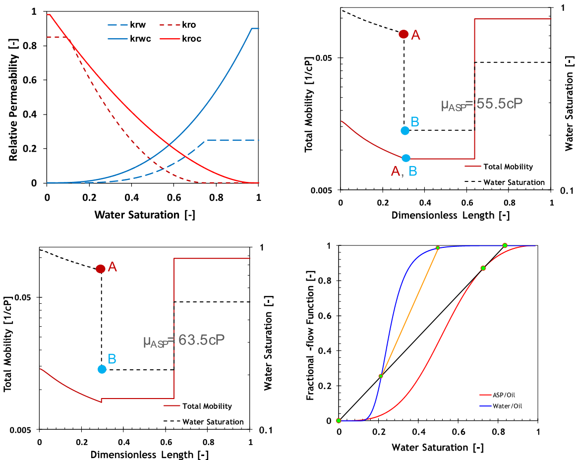
Fig. 8. The original and scaled relative permeability curves an ASP displacement IFT of 0.01 mN/m (a); water saturation and total mobility profiles (at t_D = 0.25 PV) for \mu_{ASP} = 55.5 cP (b) and \mu_{ASP} = 63.5 cP (c) obtained using method 1 and method 2, respectively. The fractional flow function vs. saturation using \mu_{ASP} = 55.5 cP (d).
