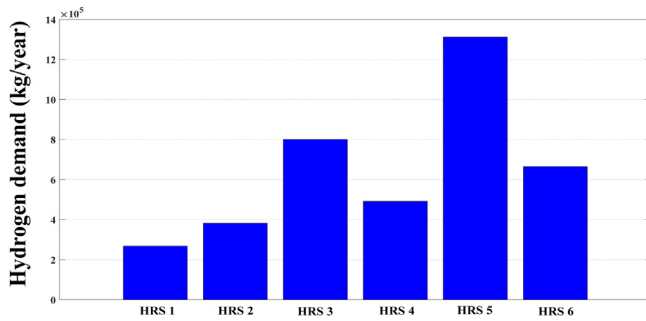
Fig. 8. Hydrogen consumption per HRS (kg/year).
