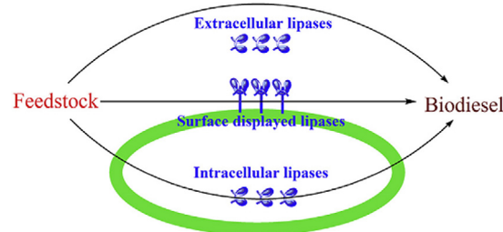
Fig. 4. Three types of genetically engineered lipases for biodiesel production (Yan et al., 2015).
