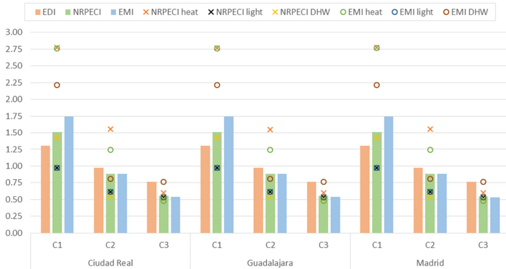
Fig. 7. Energy demand, NRPEC and EM indices (EDI, NRPECI and EMI) and disaggregated NRPECI and EMI (for heating, lighting and DHW) for climate zone D3.
