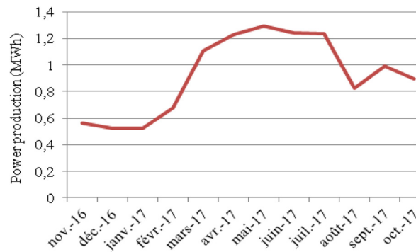
Fig. 7. Yearly variation of grid connected PV production.
