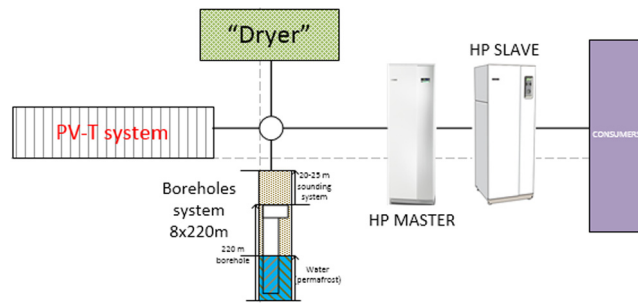
Fig. 1. Installation diagram.
