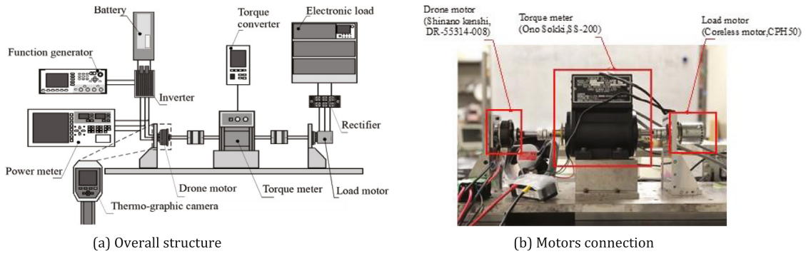
Fig. 4. Experiment configuration.
