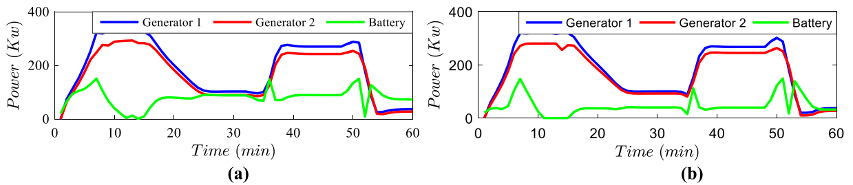
Fig. 4. (a): prediction horizon 10. (b): prediction horizon 3.
