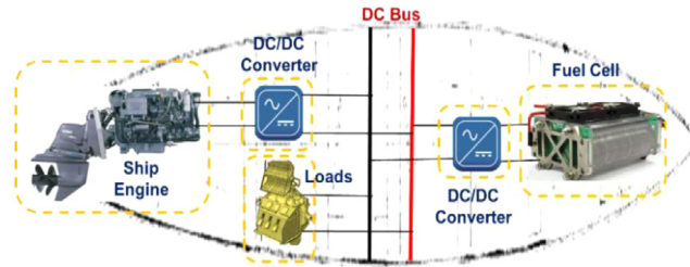
Fig. 1. The scheme of a hybrid electric ferry grid.
