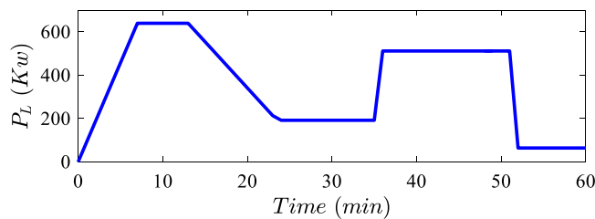
Fig. 3. Power load profile of the hybrid ferry.
