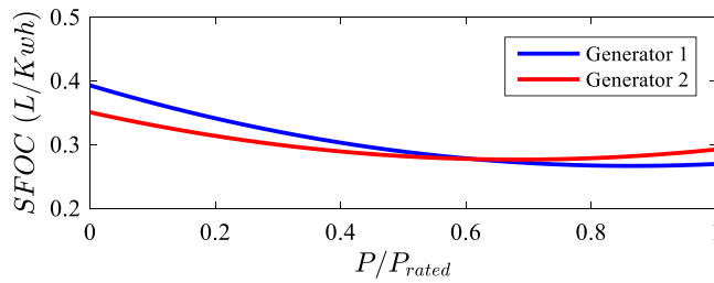
Fig. 2. The SFOC of each generator.
