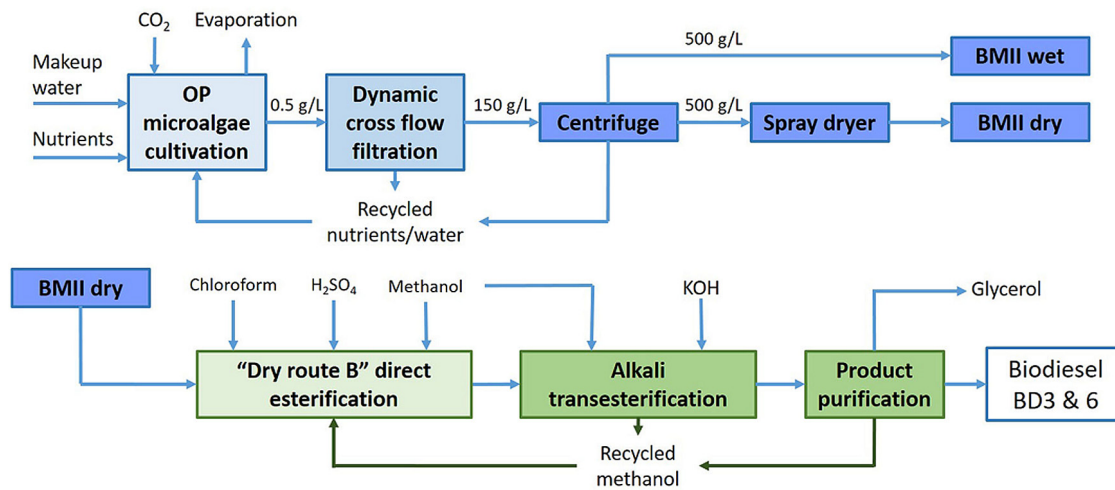
Fig. 6. Microalgae biodiesel production path (Rios et al., 2013) with permission.
