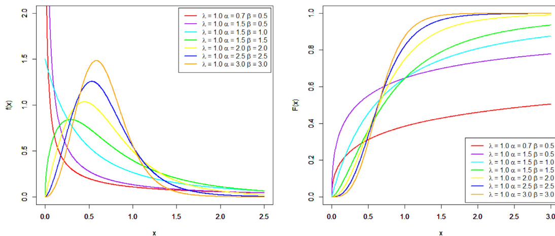
Fig. 1. PDF and CDF curves for selected parameter values.
