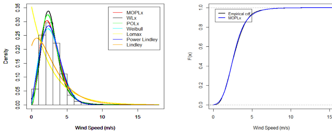
Fig. 4. The histogram and fitted density of models for wind speed data at Hariipur station.
