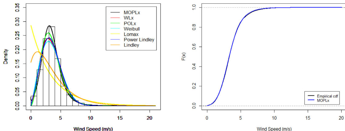
Fig. 2. The histogram and fitted density of models for wind speed data at Bahawalpur station.
