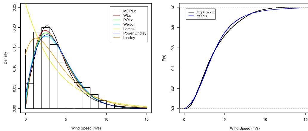
Fig. 3. The histogram and fitted density of models for wind speed data at Gwadar station.
