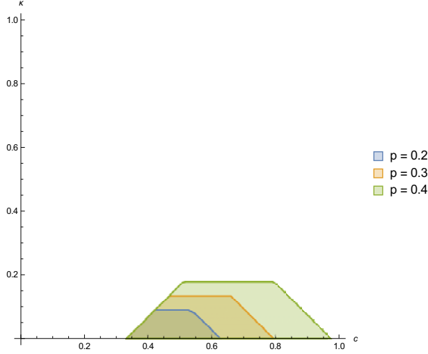
Figure 2. T_p when p \in \left\{ \frac{2}{10}, \frac{3}{10}, \frac{4}{10} \right\} .
