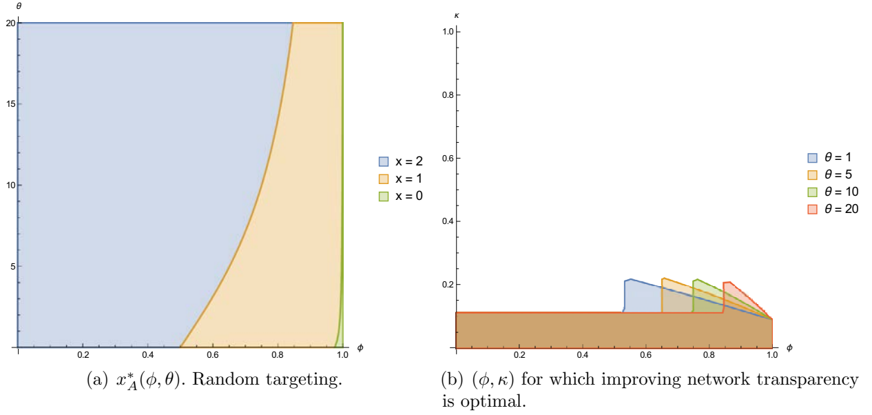
Figure 3. Robust optimal interventions.
