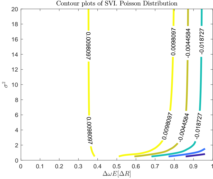
Figure 10. Optimal intervention as a function of \sigma^2 in Poisson networks with model uncertainty.
