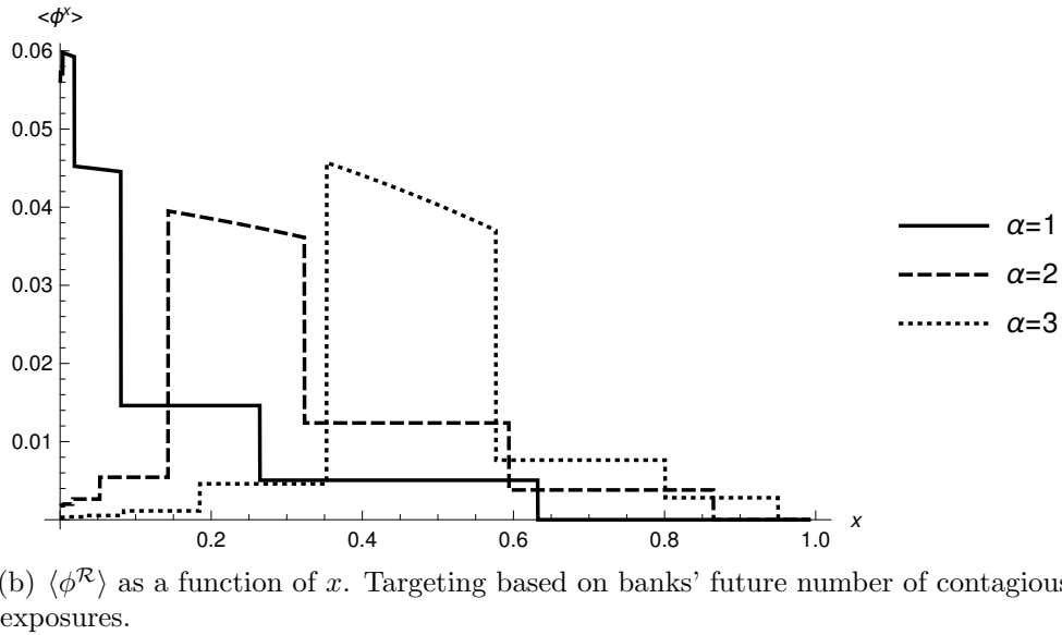
Figure 5. \{p_k\}_k follows a Poisson distribution with parameter \alpha .
