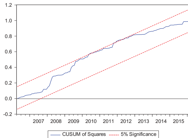
Figure 3. Result of CUSUMSQ test.
