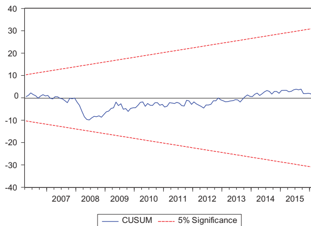
Figure 2. Result of CUSUM test.
