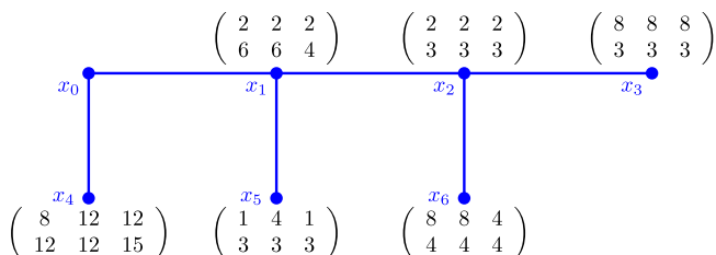
Fig. 1. The bicriteria game tree.
