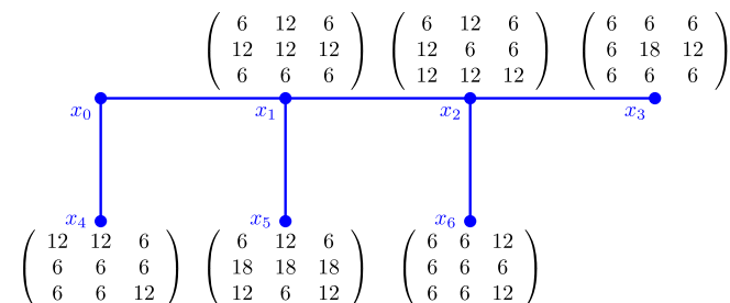
Fig. 2. The 3-criteria game tree.
