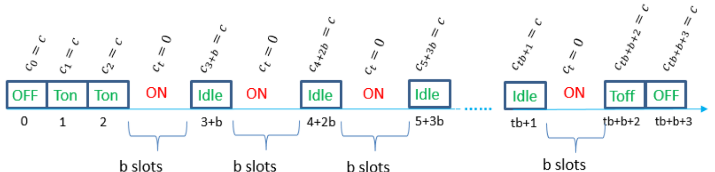
Fig. 9. An example of pb_4 which transfers to a 3-PARTITION problem.
