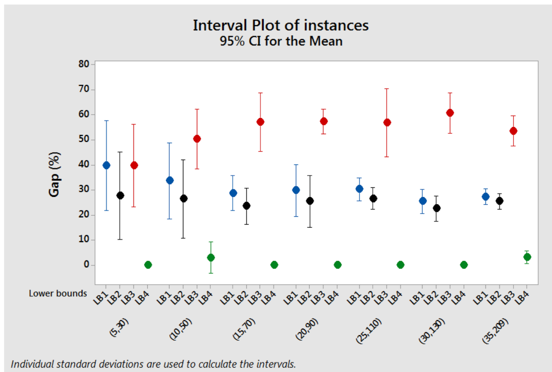
Fig. 10. Performance comparison of the lower bounds with the obtained optimal solutions by CPLEX.
