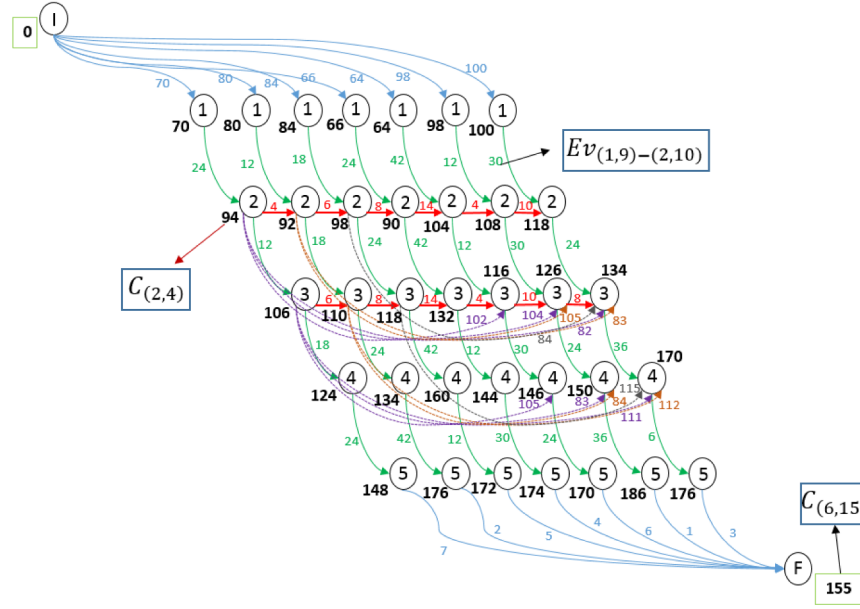
Fig. 3. The related graph for instance (3,15).
