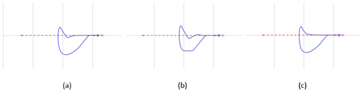
Fig. 11. Tuning Population size: trajectories of the Blue Agent with the highest fitness upon termination of the GA where the population size is 50 (a), 100 (b) and 200 (c). P_c = 0.2 , and P_m = 0.01 . Table 6 lists the remaining parameters used (For interpretation of the references to colour in this figure legend, the reader is referred to the web version of this article.).
