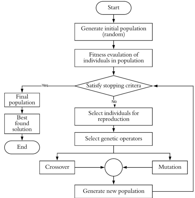
Fig. 1. Steps in a basic genetic algorithm.
