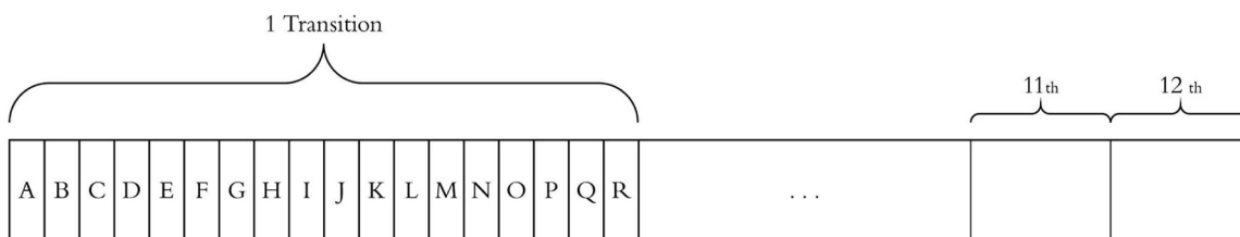
Fig. 4. Chromosome representation for evolving FSM transitions.
