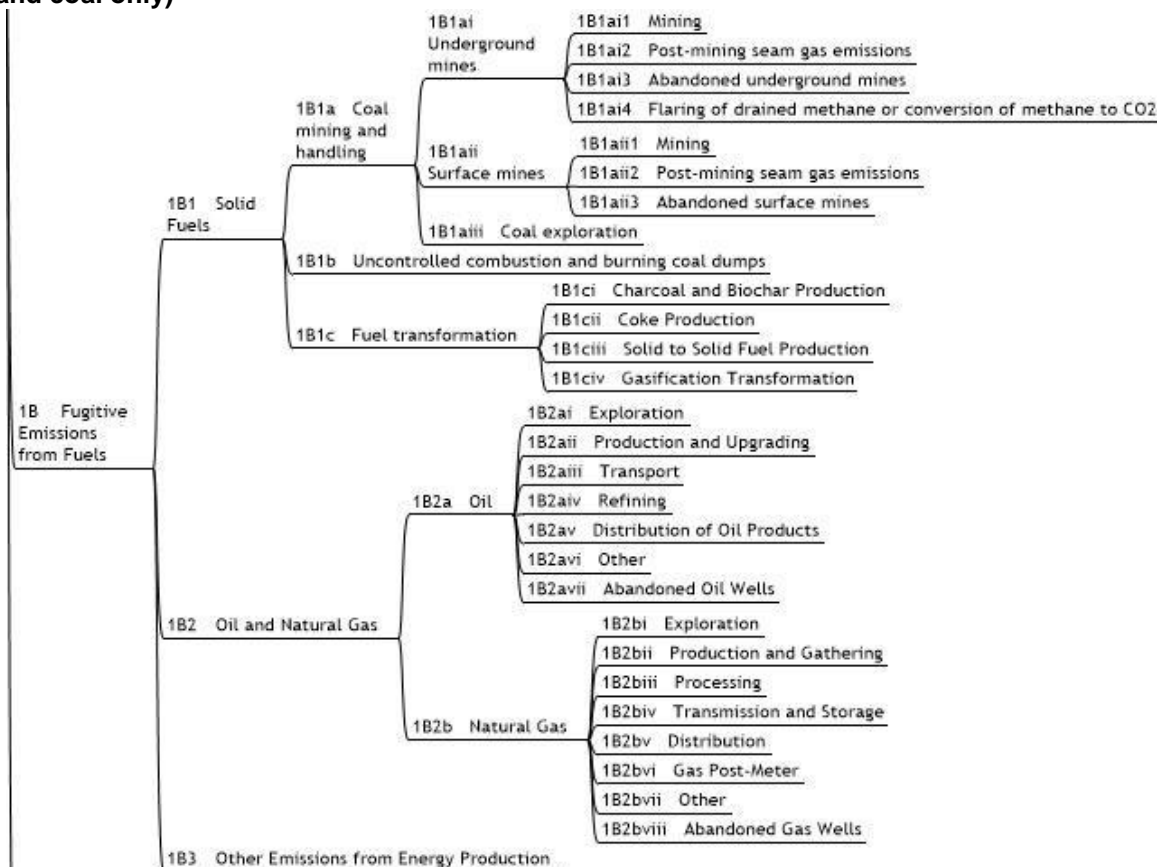
Figure 3: Fugitive Emissions from Energy Activity and Source Structure in the Energy Sector (oil, gas and coal only)*
