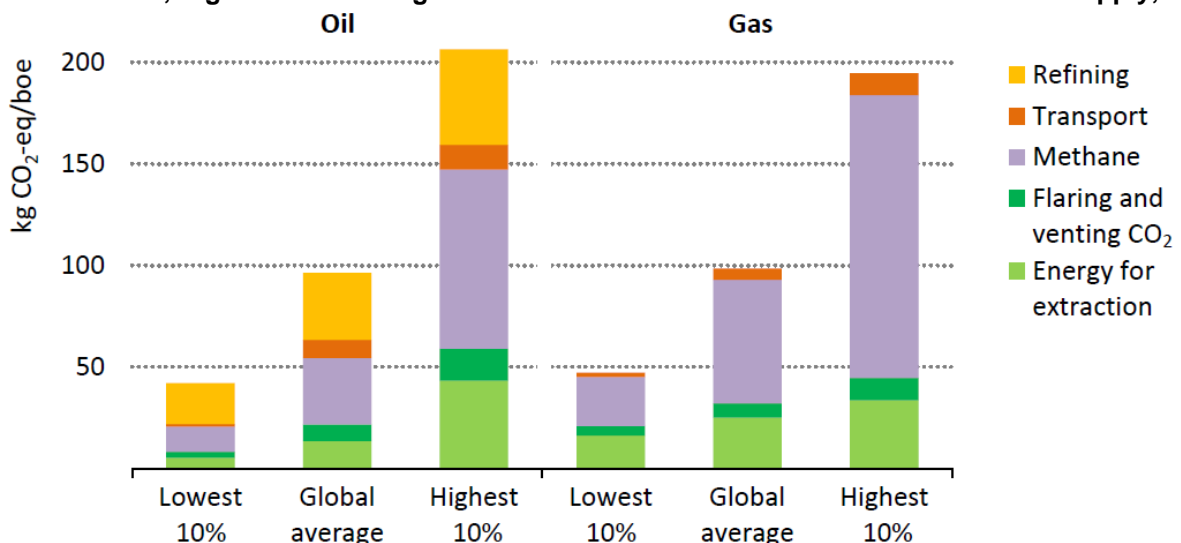
Figure 9: Lowest, Highest and Average Global GHG Emission Intensities of Oil and Gas Supply, 2017
