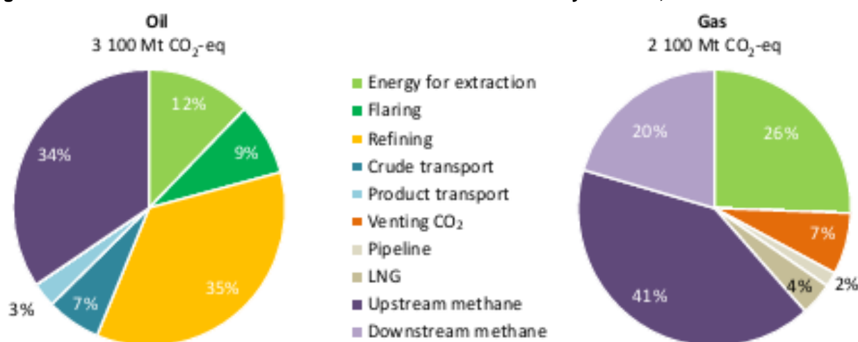
Figure 5: Breakdown of Global GHG Emissions from Oil and Gas by Element, 2017
