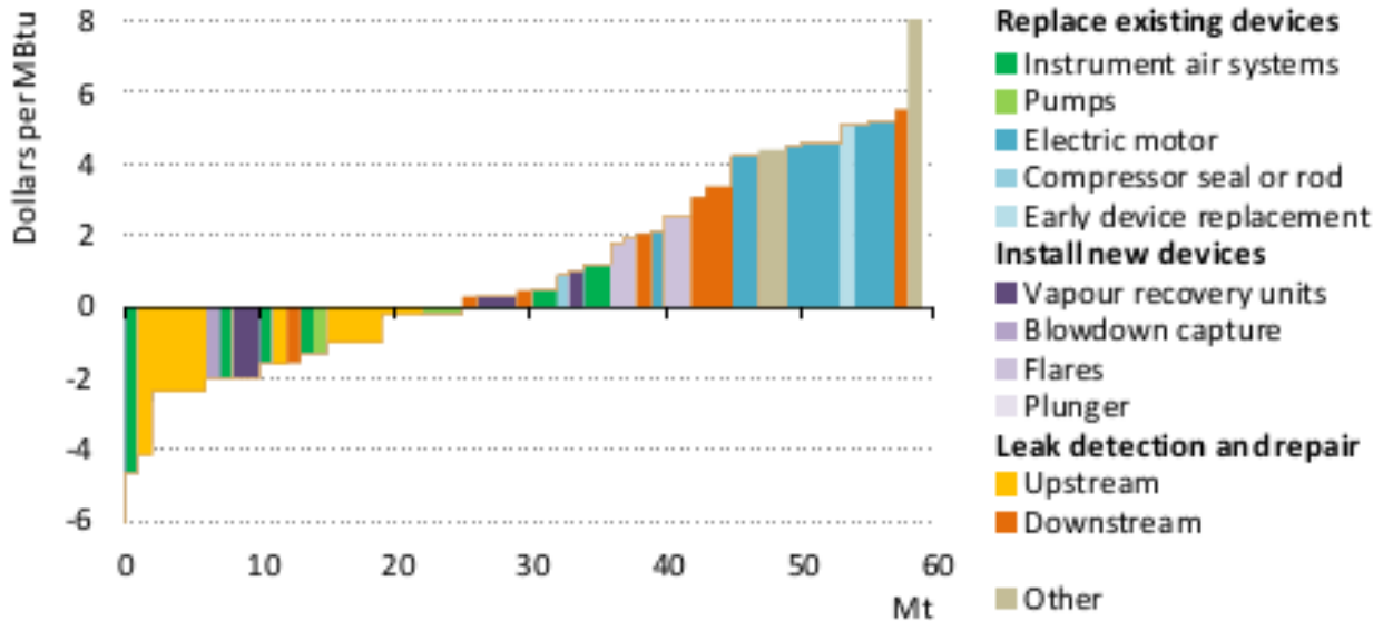
Figure 6: Abatement Costs for Oil and Gas Methane Emissions by Device and Process, 2019
