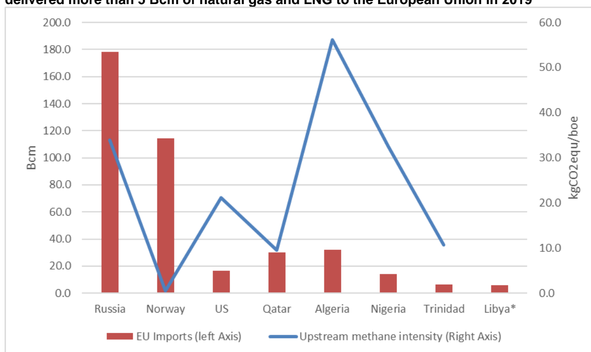
Figure 10: Methane intensity of exploration and production of oil and gas in countries which delivered more than 5 Bcm of natural gas and LNG to the European Union in 2019
