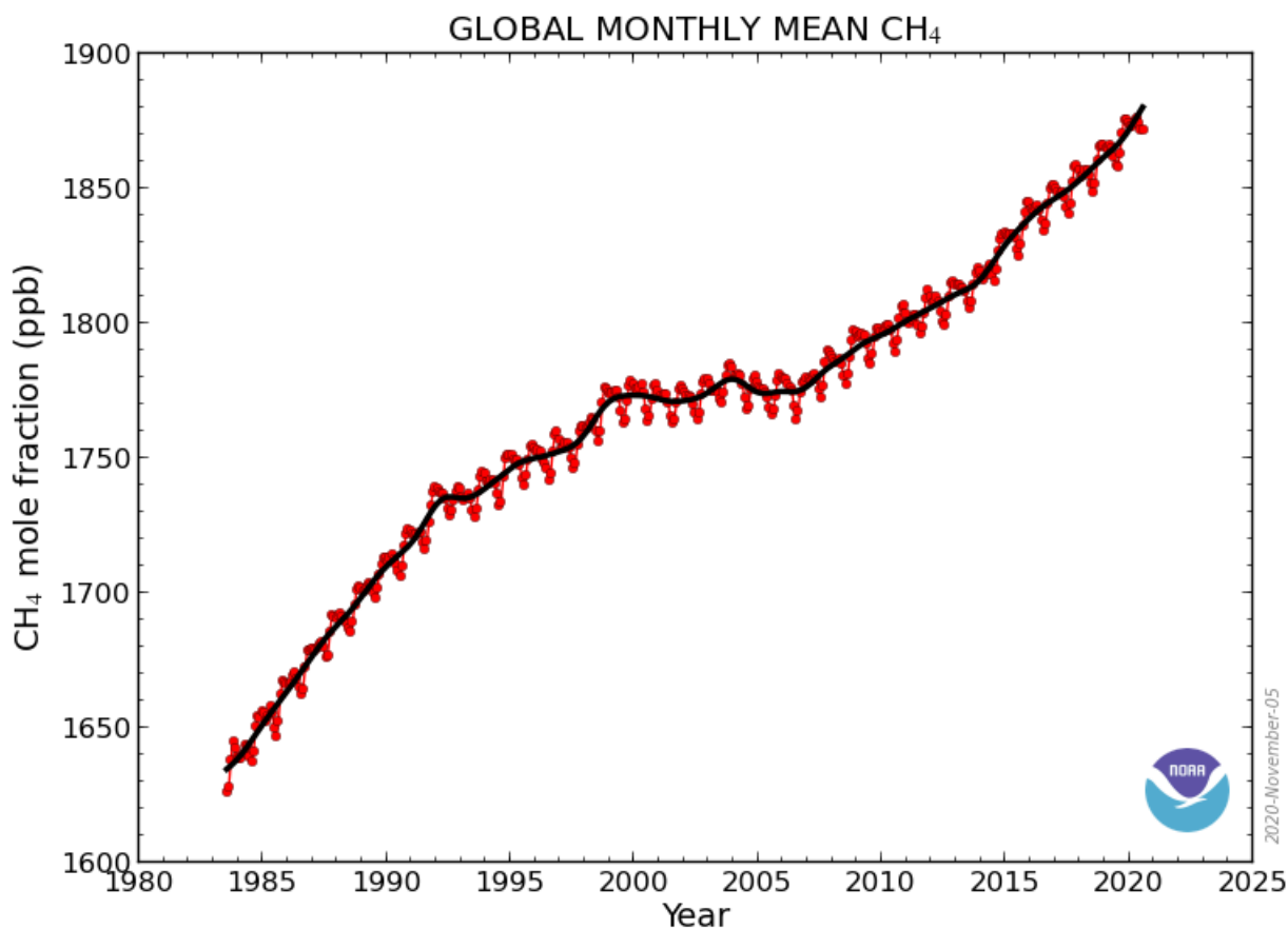
Figure 1: Global Monthly Mean Atmospheric Methane Levels 1980-2020
