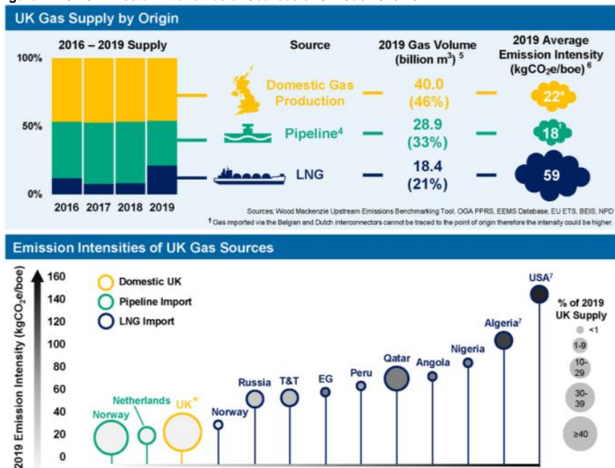
Figure 12: GHG Emission Intensities of Sources of UK Gas 2016-19
