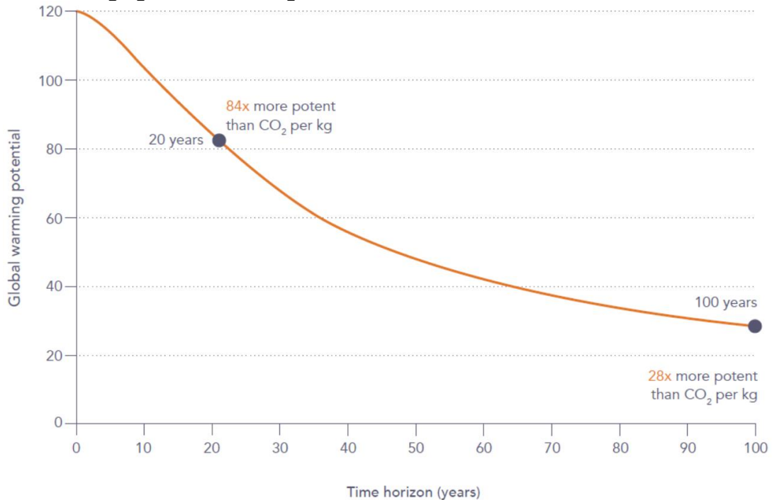
Figure 2: The Changing Global Warming Potential of Methane over Time
