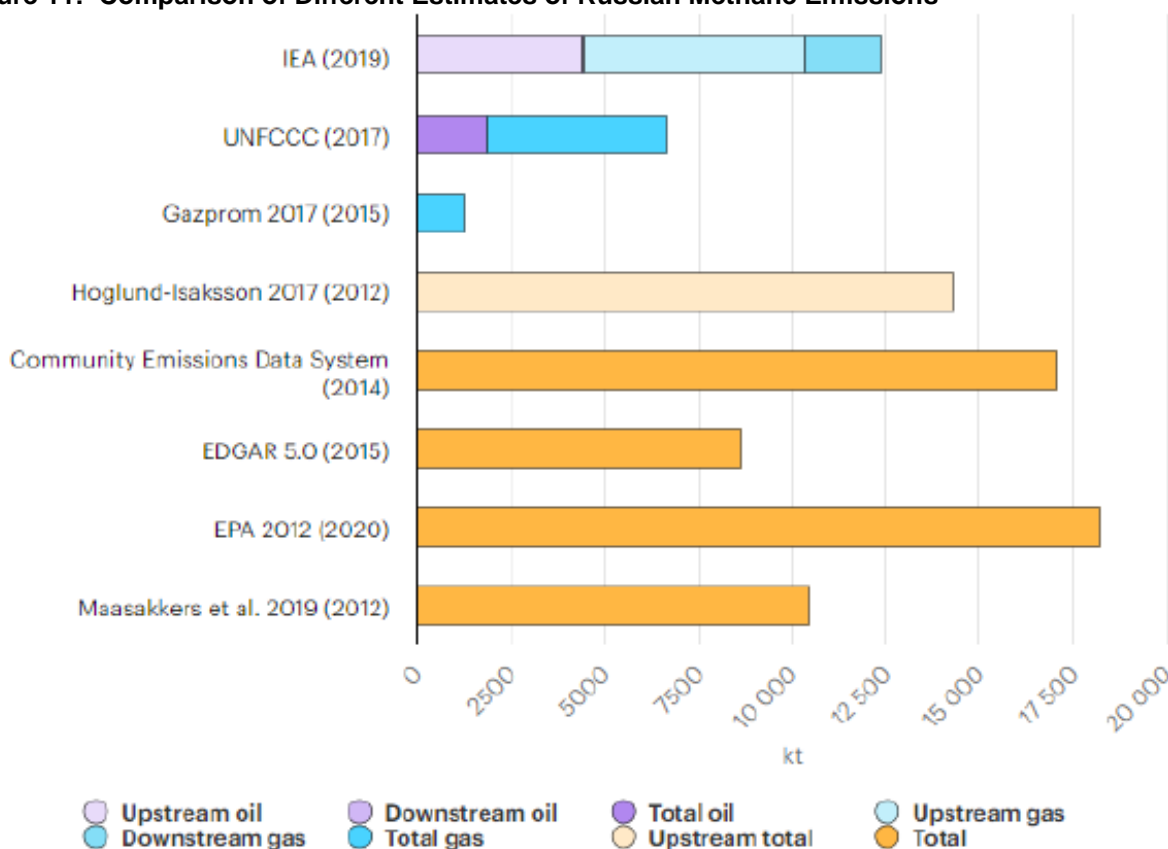
Figure 11: Comparison of Different Estimates of Russian Methane Emissions
