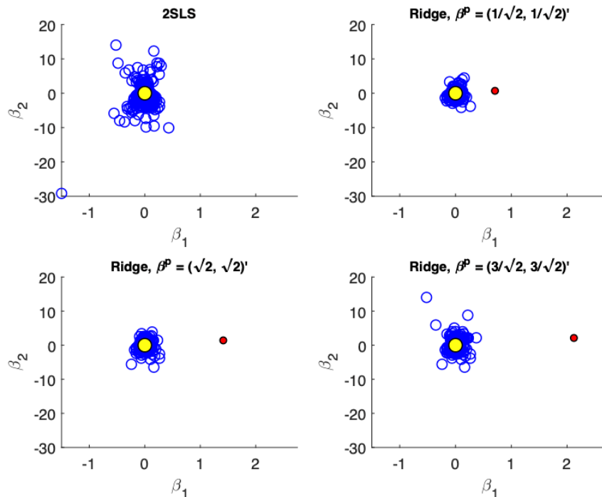
Figure 2. Scatter plots of the estimates from TSLs and ridge estimator with different priors when precision is low ( \delta = 0.1 ) and sample size is large ( n = 500 ). Estimates, the true parameter value and prior values are represented by blue, yellow and red points respectively. The variance associated with TSLs estimates is much larger than the ridge estimates. The ridge estimator is less biased towards the prior in the larger samples.
