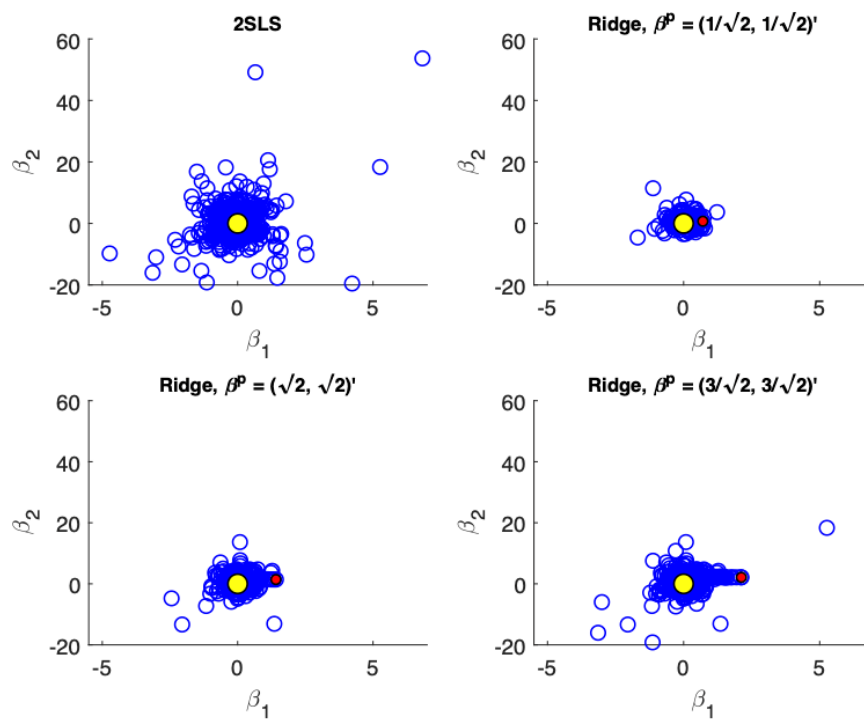
Figure 1. Scatter plots of the estimates from TSLs and ridge estimator with different priors when precision is low ( \delta = 0.1 ) and sample size is small ( n = 25 ). Estimates, the true parameter value and prior values are represented by blue, yellow and red points respectively. The variance associated with TSLs estimates is much larger than the ridge estimates. The ridge estimator is biased toward the prior.
