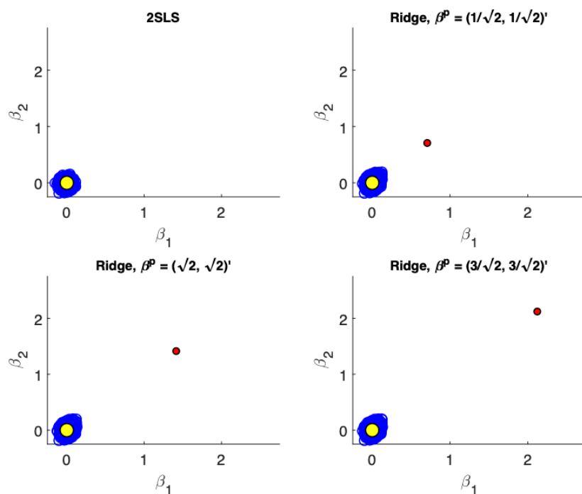
Figure 4. Scatter plots of the estimates from TSLS and ridge estimator with different priors when precision is high ( \delta = 1 ) and sample size is large ( n = 500 ). Estimates, the true parameter value and prior values are represented by blue, yellow and red points respectively. The TSLS estimates outperform the ridge estimators which is demonstrated by marginally larger clouds which are slightly off-center from the true parameter values for the ridge estimators. However, the ridge estimator using different priors is still competitive.
