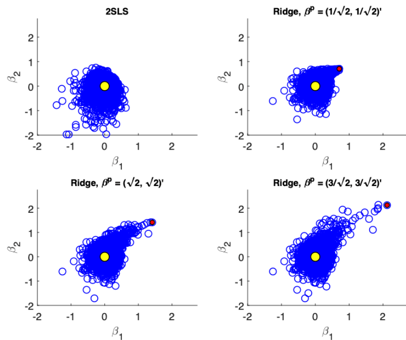
Figure 3. Scatter plots of the estimates from TSLS and ridge estimator with different priors when precision is high ( \delta = 1 ) and sample size is small ( n = 25 ). Estimates, the true parameter value and prior values are represented by blue, yellow and red points respectively. TSLS performance is much better in this setting. The variance reduction for the ridge estimator is not as dramatic.
