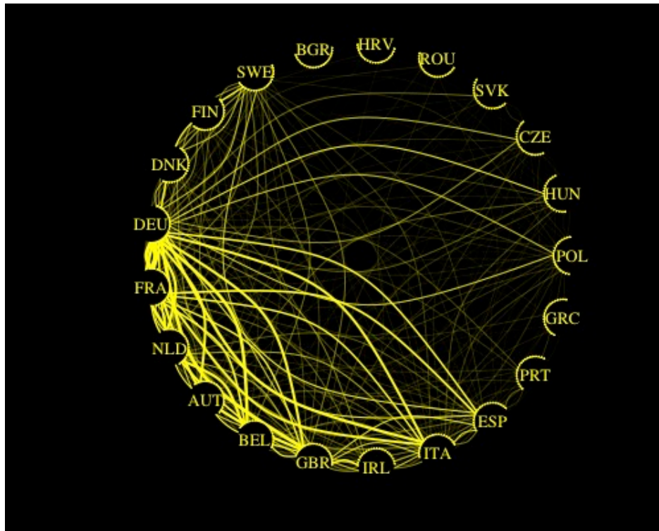
Figure 1 – Backward linkages network over time 2000 and 2014
