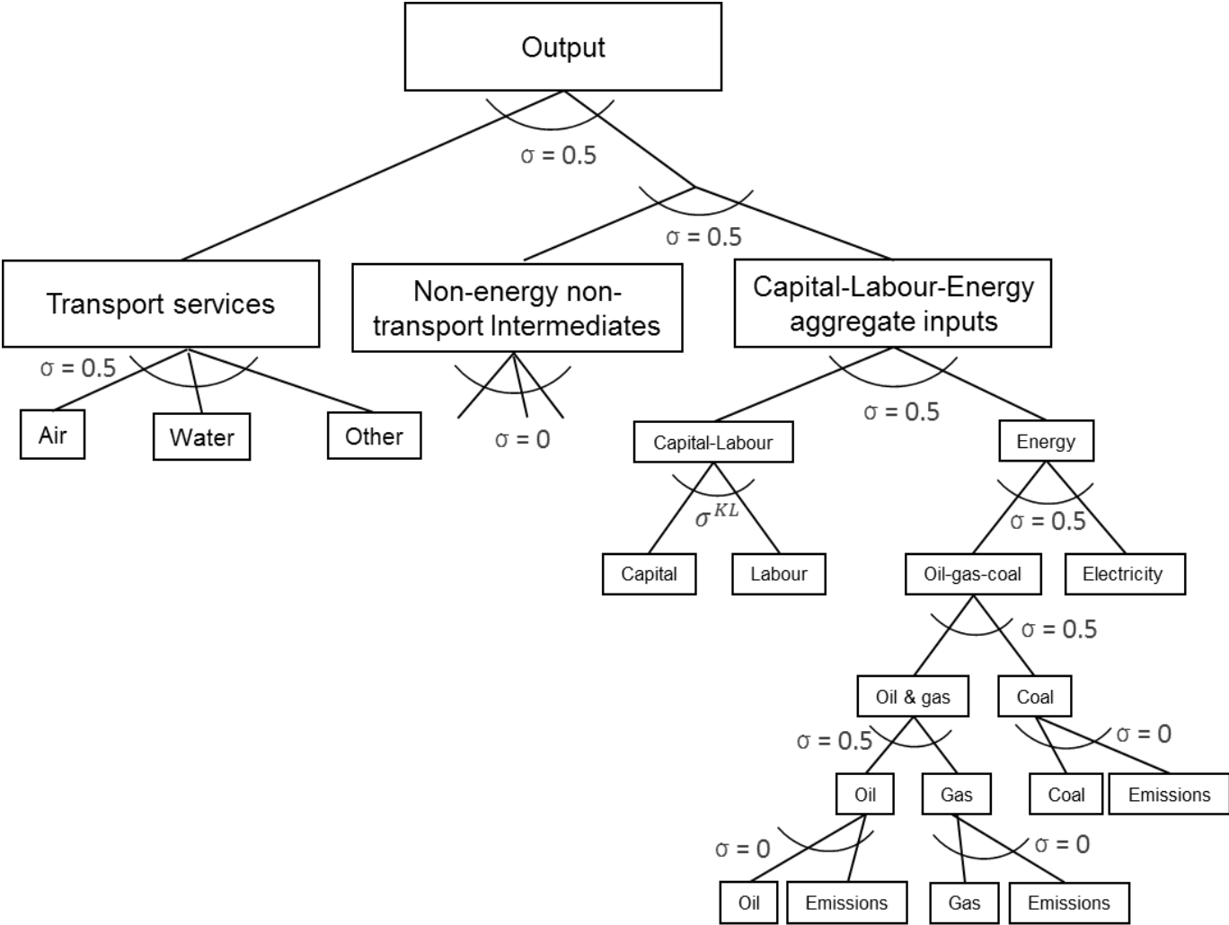
Figure 4. Nested CES structure of production technology for non-fossil fuel extraction industries
