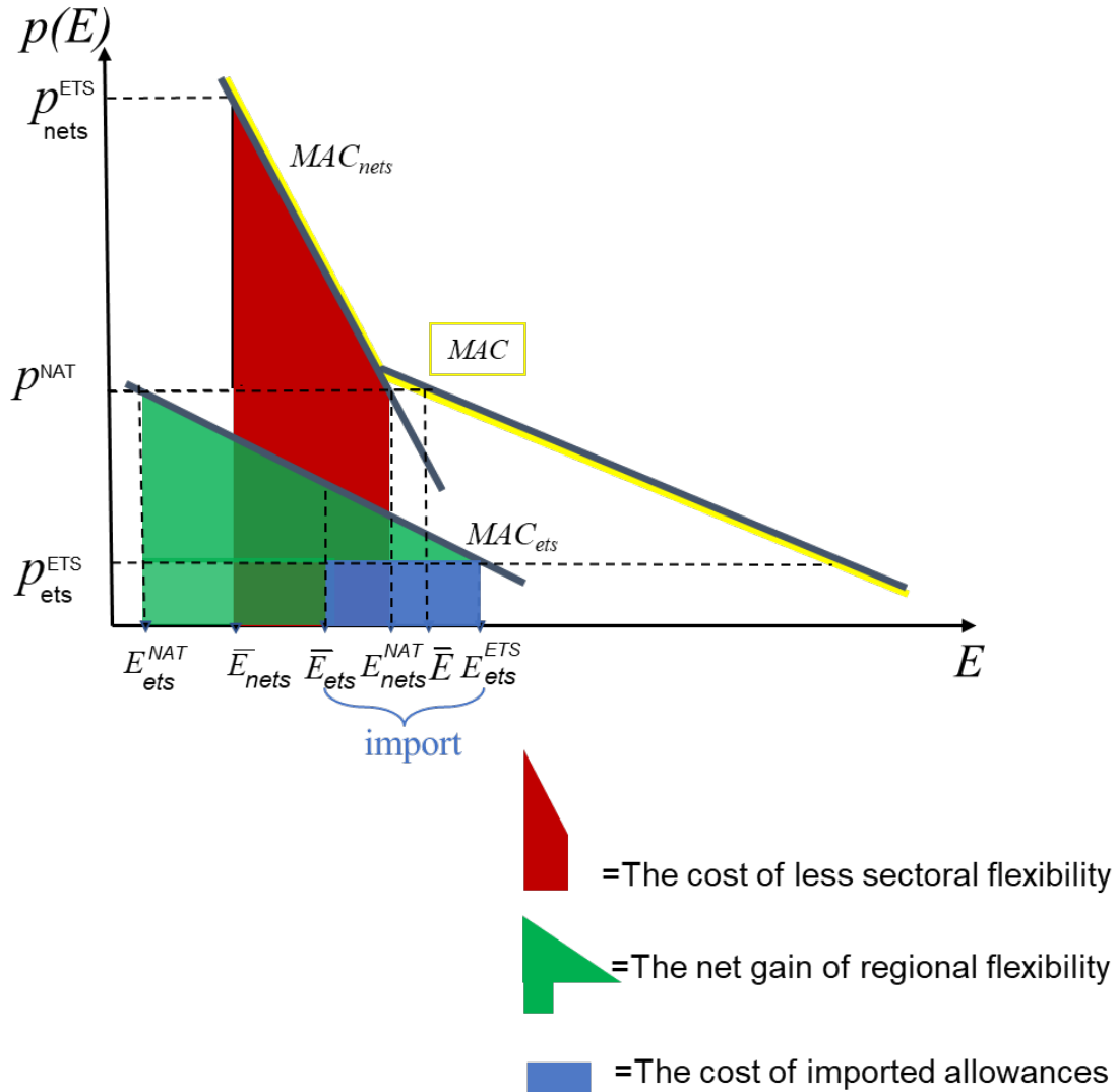
Figure 2: Net abatement cost impact for the small country in the hybrid ETS regime vs. the national cap-and-trade regime, NAT
