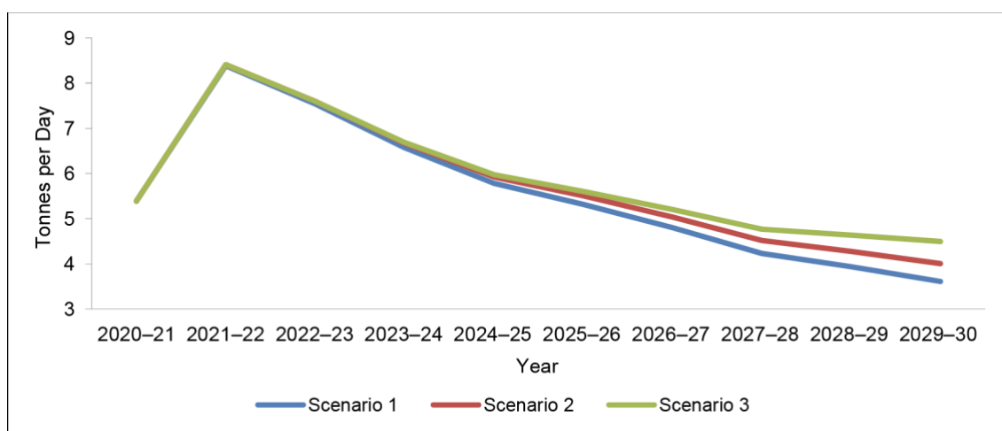
Figure 1: PM Emissions from Vehicles (2020–2030)
