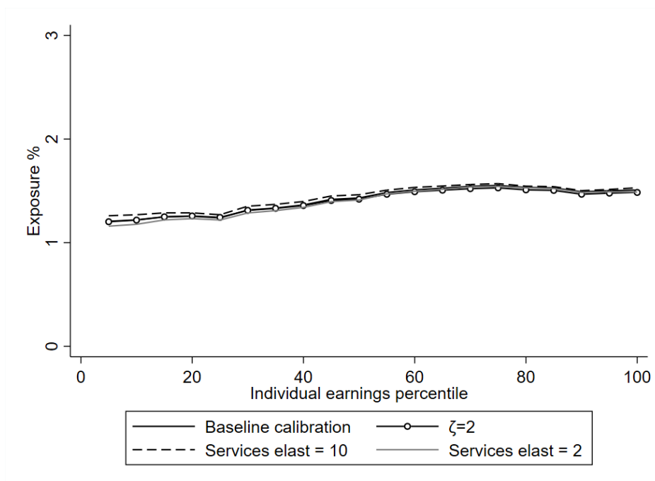
Figure B.3: Measures of response-inclusive exposure over the earnings distribution: different modelling assumptions
