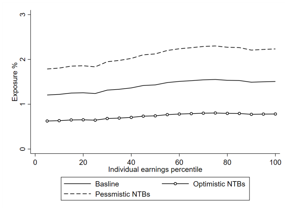
Figure B.1: Measures of response-inclusive exposure over the earnings distribution: different assumptions on non-tariff barriers
