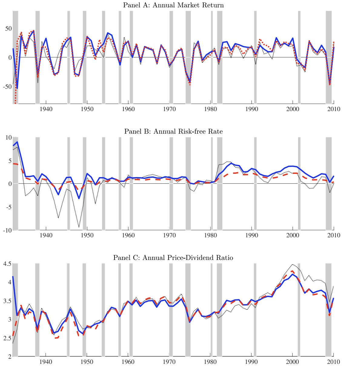
FIGURE 3: Estimated Latent States
