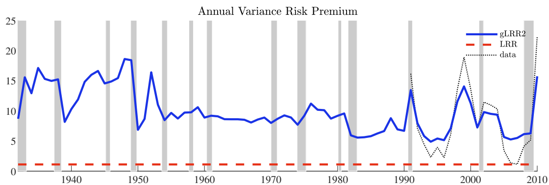
FIGURE 2: The Variance Premium in the Data and Models
