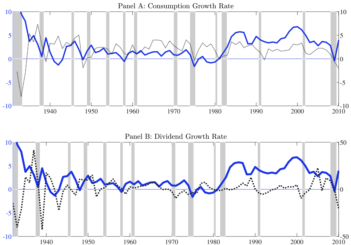
FIGURE 4: Estimated Latent States
