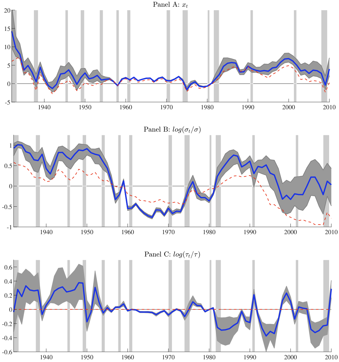
FIGURE 1: Estimated Latent States
