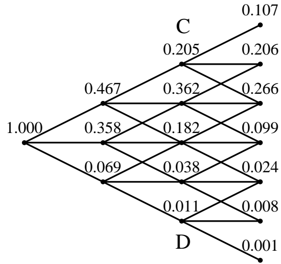
Figure 12: Arrow-Debreu prices for \sigma_I = 0.11 - \Delta K \cdot 0.005 . Nodes C and D had inadmissible transition probabilities (21)–(24).
