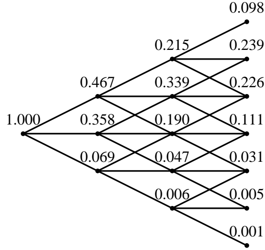
Figure 9: Arrow-Debreu prices for \sigma_I = 0.11 - \Delta K \cdot 0.001 .
