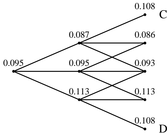
Figure 13: Implied local volatilities for \sigma_I = 0.11 - \Delta K \cdot 0.005 . Nodes C and D had inadmissible transition probabilities (21)–(24).
