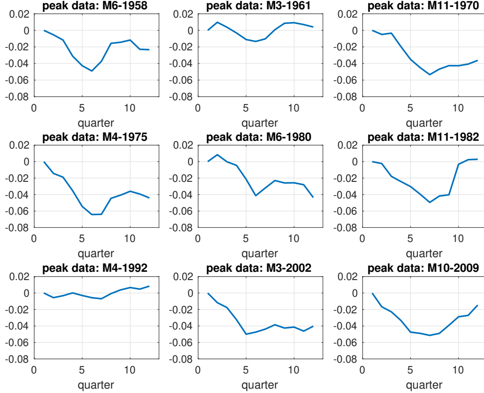
Figure 12: Exogenous shocks shifting the Beveridge curve
