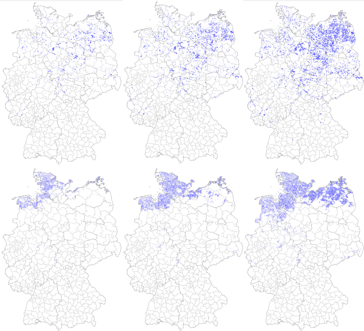
Figure 5: Wind turbine placement for expansion targets of 25 GW (left), 50 GW (middle), and 100 GW (right) for optimal (upper maps) and sub-optimal (lower maps) placement
