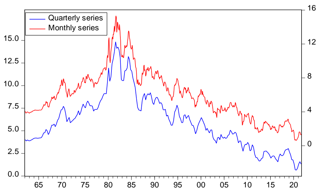
Figure 1: Quarterly and Monthly 10-year US Treasury bond yields
