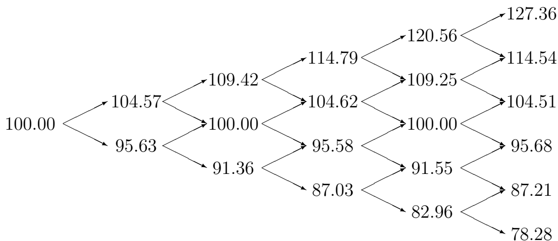
Figure 10.4. Stock price tree calculated with the DK algorithm with S_0^0 = 100 , r = 0.03 and T = 1 year.
