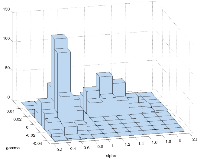
Figure 1: Prior distribution
