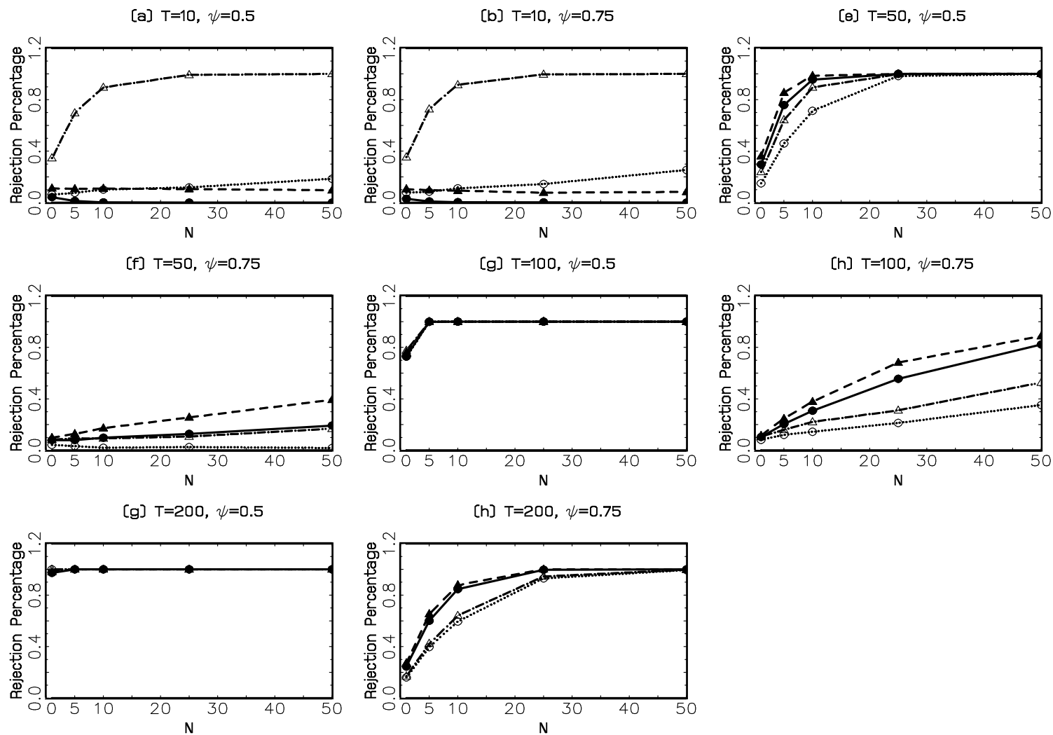
Figure 5: Empirical power results of the tests for DGP B and true cointegrating rank of two when hypothesized rank is one. ●—— panel SL-asym, ▲ — — — panel SL-VAR(1), ○..... LLL-asym, △ - · - · - LLL-VAR(1).
