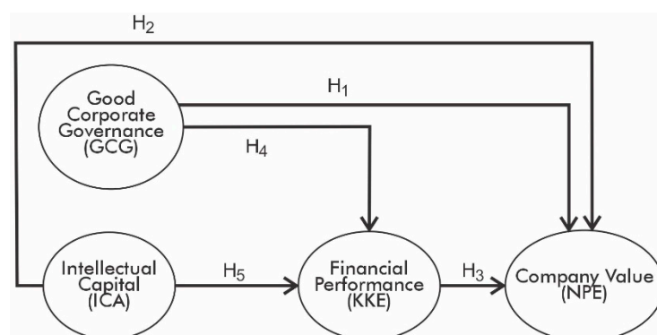
Figure 1. Research model.
