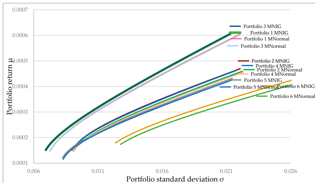
Figure 1. Efficient frontier curves for portfolios (described in Table 3) considering the MNIG and Empirical sample (MNNormal) variance-covariance matrix. Elaborated by authors with data from Bloomberg.
