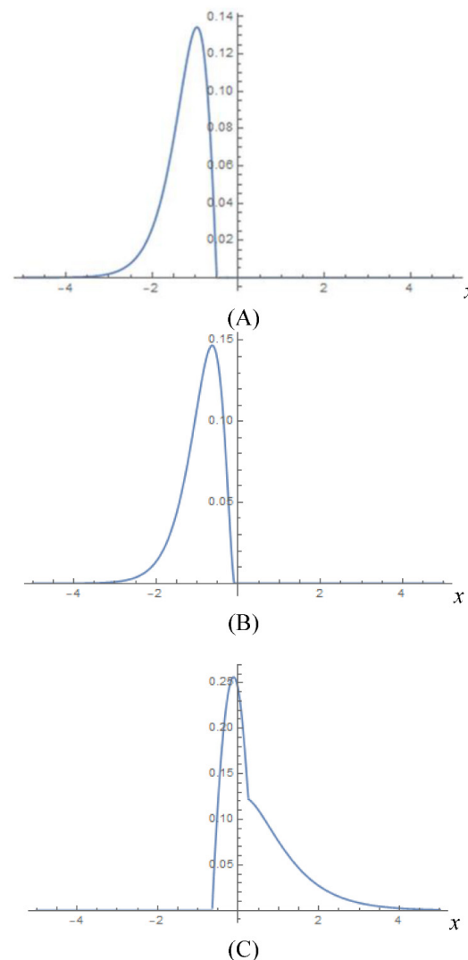
Figure 3. The shape of the pulse in arbitrary units (a response to the delta function) in the cases (A) \tau = x/c - 0.5a , (B) \tau = x/c - 0.25a , and (C) \tau = x/c + 0.25a . The spatial coordinate is measured in the units c \cdot a (see Equation (5)).
