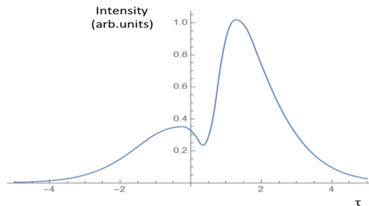
Figure 4. Autocorrelation of the square of the Green function kernel I(\tau) = \int_{-10}^{10} K^2\left(x, \frac{x}{v} - \tau\right) dx (see Equation (14) in the text), as a function of time delay and v = 0.75c . Limits of integration are arbitrary as a truncation to approximate [-\infty, +\infty] with the necessary accuracy.
