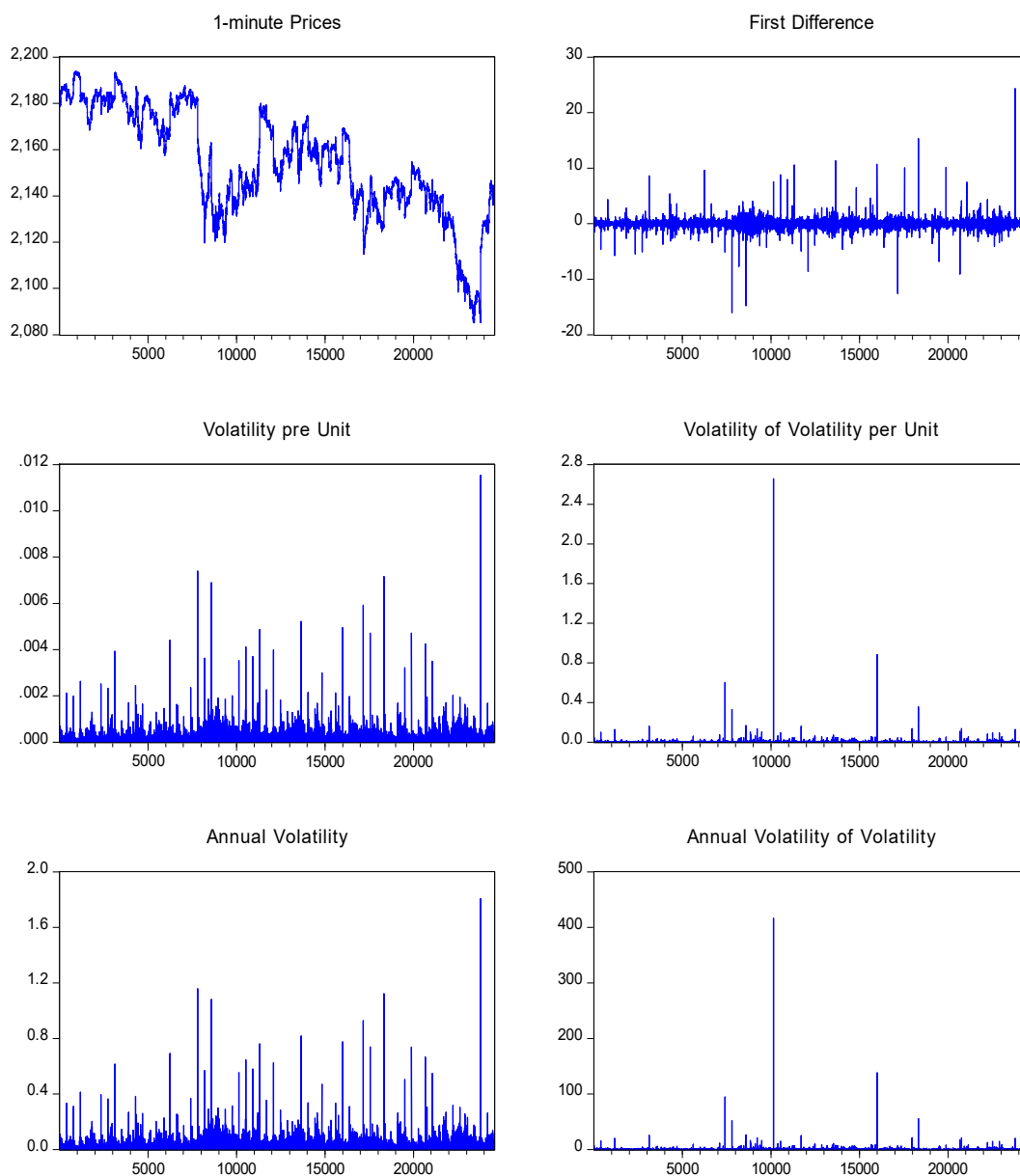
Figure 1. Plot of the S&P 500 1-min sample.
