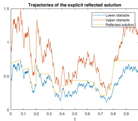
Figure 9. One path of Y^{\tau, \kappa} in the explicit reflected scheme ( \tau = 0.2 ).
