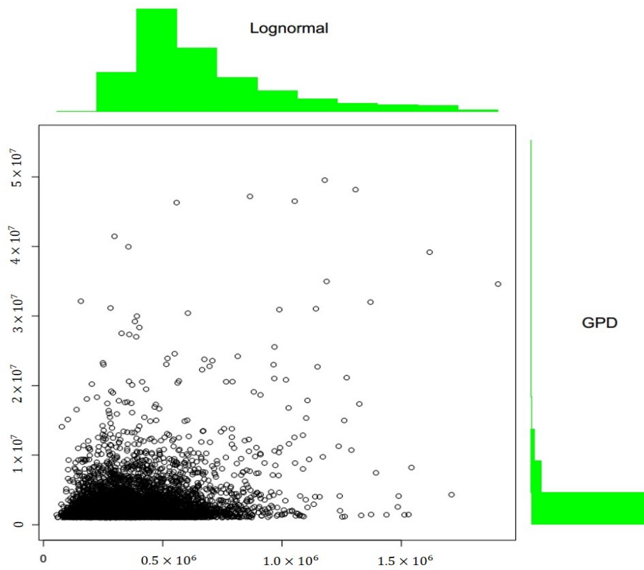
Figure 11. Lognormal (top) and GPD (right) marginal histograms and Gumbel Copula simulated values plot.
