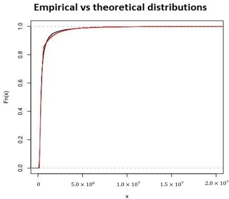
Figure 9. Lognormal–GPD–Gamma (red) versus empirical (dark) distribution functions.
