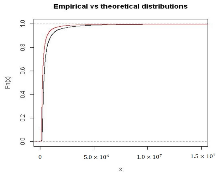
Figure 4. Lognormal–Burr and empirical distribution functions (red and dark lines).
