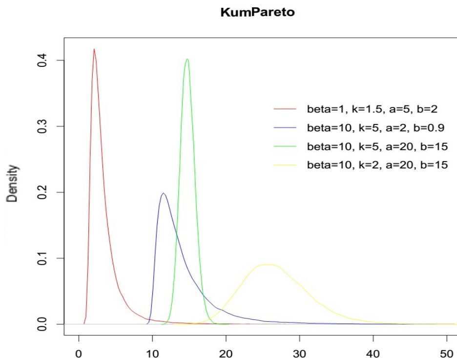
Figure 2. KumPareto density functions.
